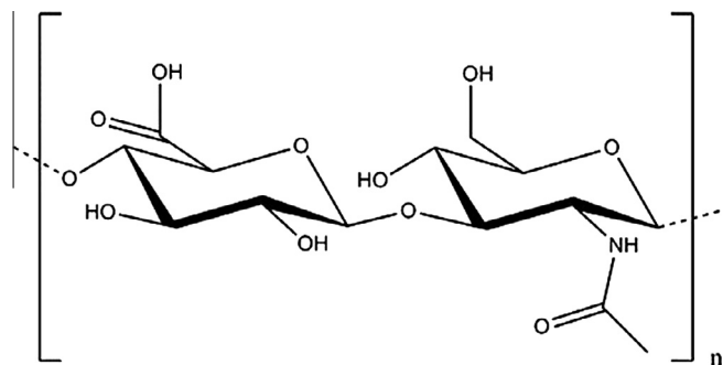
Fig. 1. Chemical structure of HA, which is made of disaccharide repeats of N -acetylglucosamine and glucuronic acid.
