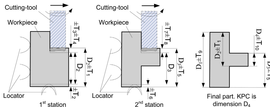
Fig. 1. Example of the influence of machining-induced variations on the tolerance allocation problem.
