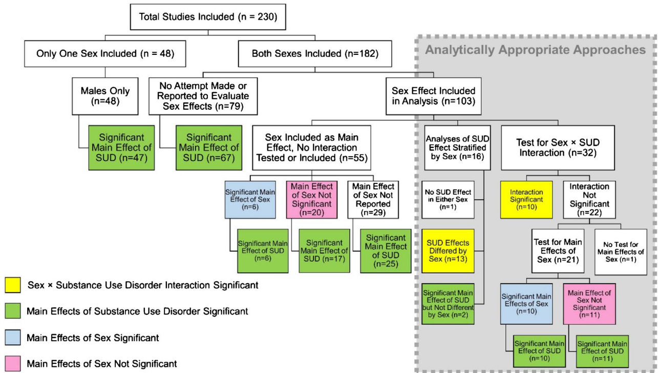
Fig. 2 Evaluation Results of Statistical Methodology.
