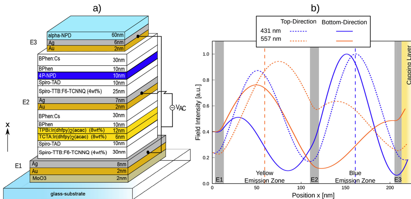
Fig. 1. a) Schematic stack architecture with layer thicknesses and contacting of the AC/DC OLED. b) Distribution of the electric field in the device. 431 nm and 557 nm refer to the PL-peak intensity of the blue and yellow emitter, respectively. The emission zones are located in the field maximum for both colors and emission directions. (For interpretation of the references to colour in this figure legend, the reader is referred to the web version of this article.)
