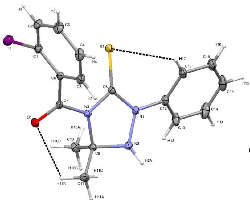
X-ray structures of 1,2,4-Triazole and Triazolidin derivatives
