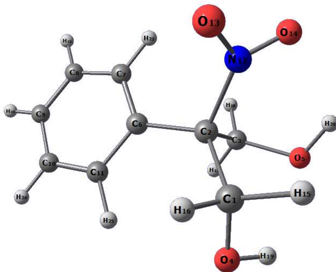
2-Nitro-2-Phenyl-Propane-1,3-Diol
