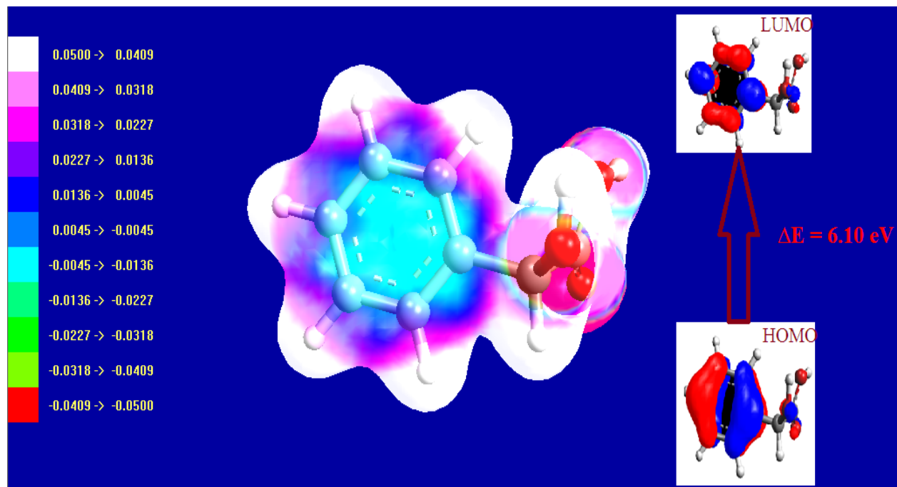
Figure shows molecular electrostatic potential and HOMO-LUMO energy of DLMA.
