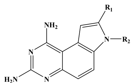
7,8-dialkyl-1,3-diaminopyrrolo-[3,2-f] Quinazoline derivatives
