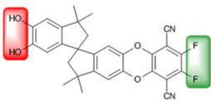
AB-type monomer
