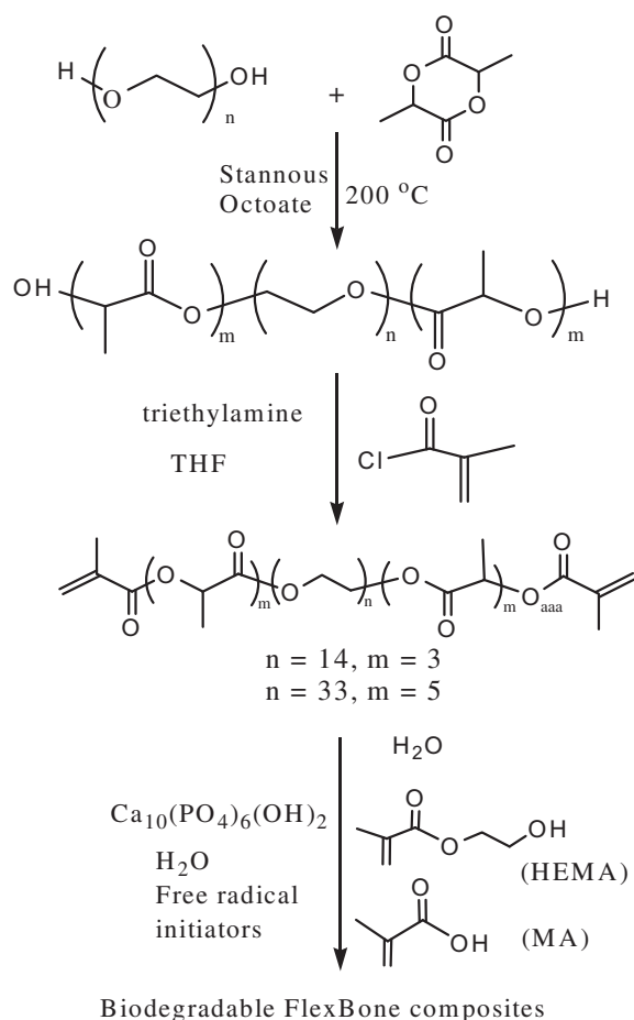
Scheme 1. Synthesis of degradable macromers and poly(HEMA-co-MA)/HA biocomposites.
