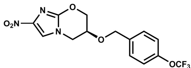
PA-824 ( 34 )
