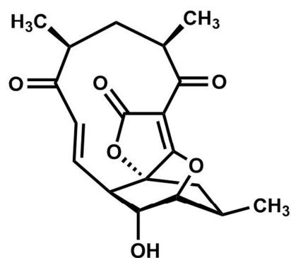
abyssomicin C ( 32 )
