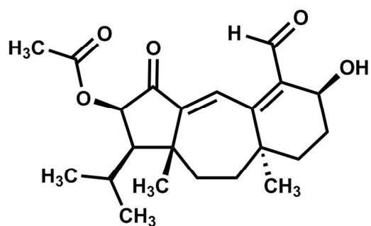
guanacastepene A ( 29 )
