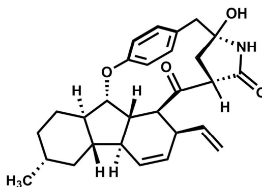
hirsutellone B ( 30 )
