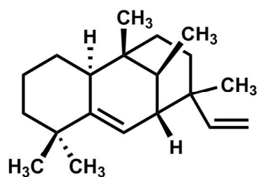
"edaxadiene" ( 33 ) (originally reported strucutre)
