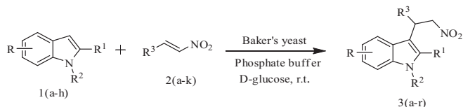
Scheme 1. Michael addition of indoles to nitroolefins in fermented baker's yeast at room temperature.
