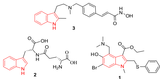
Figure 1. Bioactive compounds containing 3-substituted indole nucleus.
