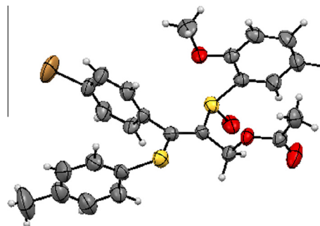
Figure 1. ORTEP diagram of compound 6 .
