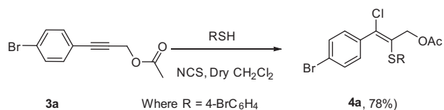
Scheme 1. Chlorothiolation of internal alkyne.
