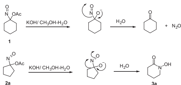
Scheme 1. Pathways of acyloxy nitroso compound hydrolysis.
