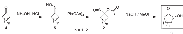
Scheme 2. Conversion of ketones to cyclic hydroxamic acids via acyloxy nitroso compounds.
