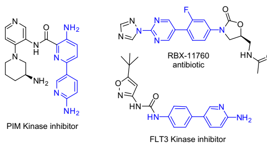
Figure 1. Bioactive molecules with hetero-biaryl systems.
