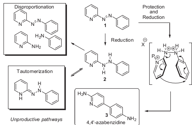
Scheme 1. Tautomerization of N -phenyl- N' -pyridin-2-ylhydrazine.
