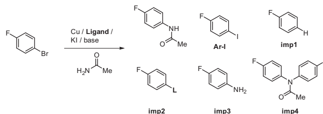
Scheme 1. Cu-catalyzed cross-coupling of acetamide and 4-bromofluorobenzene.
