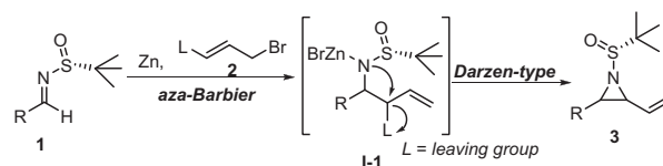
Scheme 1. Reaction proposal.
