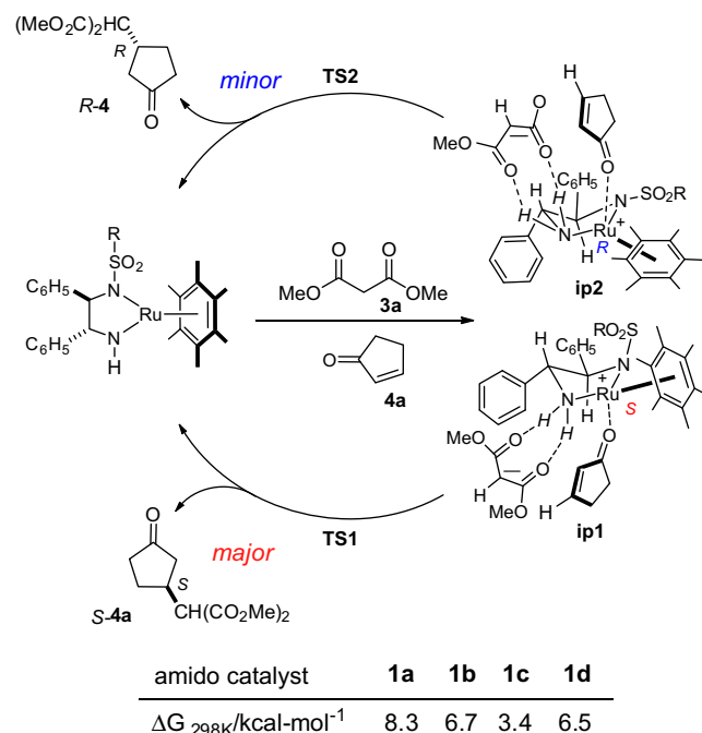
Scheme 2. Sense of the enantioselection within the proposed mechanism. Difference of the computed C-PCM free energies (298 K) of the R- and S-pathways, ΔG o = G(TS2) 298 K - G(TS1) 298 K , kcal/mol -1 .
