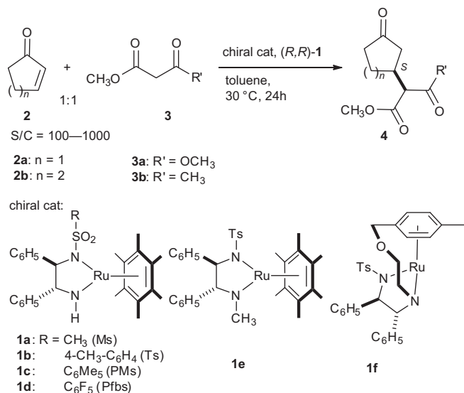
Scheme 1. Asymmetric C–C bond formation with chiral amido catalysts.
