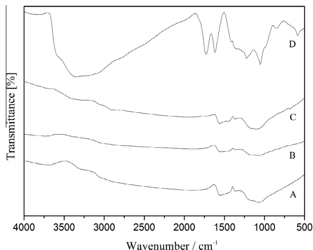
Figure 1. FT-IR of pristine rGO-1, (A) rGO-1 after being used one time, (B) rGO-1 after being used five times, (C) and GO (D).
