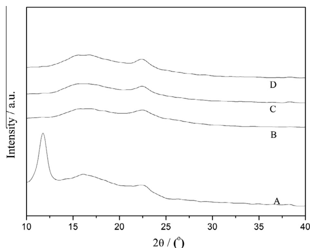
Figure 2. XRD patterns of GO, (A) pristine rGO-1, (B) rGO-1 after being used one time, (C) and rGO-1 after being used five times (D).
