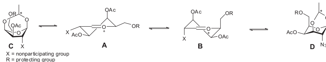
Scheme 1. Mechanism of the remote protecting group directing effect.
