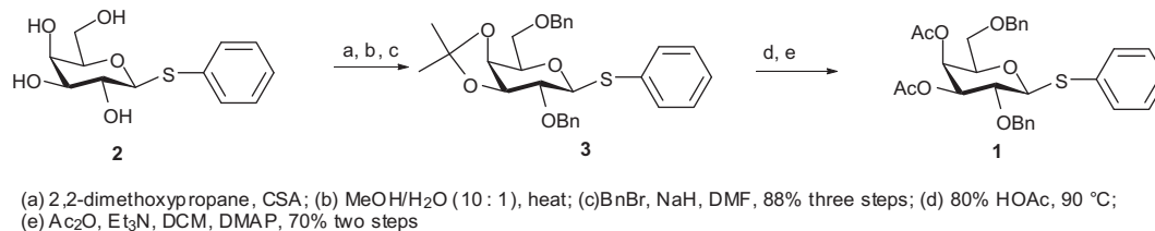
Scheme 2. Preparation of donor 1 .
