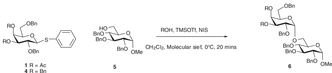
Scheme 3. Glycosylation reaction with acceptor 5 .
