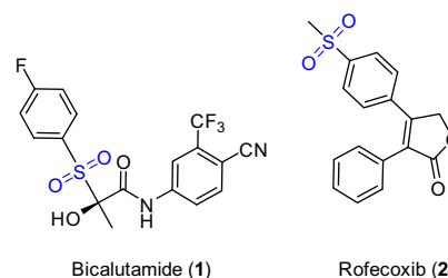
Figure 1. Commercial sulfone containing drugs.
