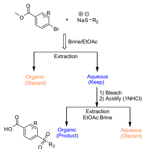
Scheme 1. Flow chart for S_NAr -oxidation protocol.
