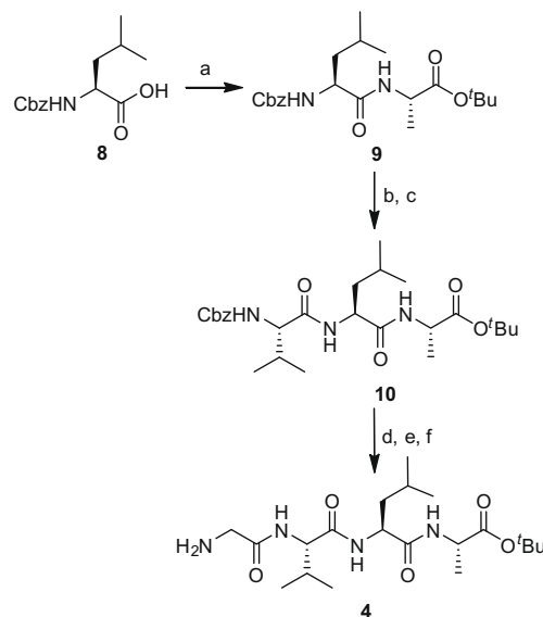
Scheme 2. Reagents and conditions: (a) H-Ala-O t Bu, EDCI, HOBT, CH 2 Cl 2 , 12 h, 80%; (b) Pd/C (10%), H 2 , EtOAc, 2 h; (c) Cbz-Val-OH, EDCI, HOBT, CH 2 Cl 2 , 14 h, 76%; (d) Pd/C (10%), H 2 , EtOAc, 2 h; (e) Cbz-Gly-OH, EDCI, HOBT, CH 2 Cl 2 , 18 h; (f) Pd/C (10%), H 2 , MeOH, 3 h, 64% over three steps.
