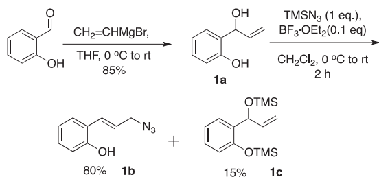
Scheme 3. Synthesis of allylic azide and disilylated product.
