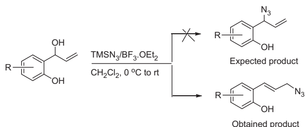
Scheme 1. Synthesis of allylic azides from aryl vinyl carbinols.
