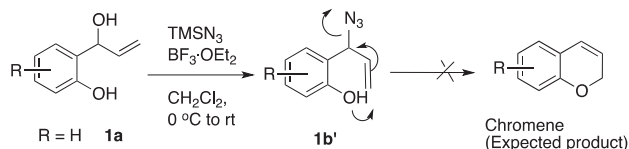
Scheme 2. Attempted nucleophilic substitution reaction towards chromene formation.
