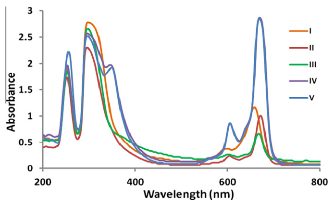
Figure 1. UV/Vis absorption spectra of I–V in THF ( c = 3 \times 10^{-5} M).
