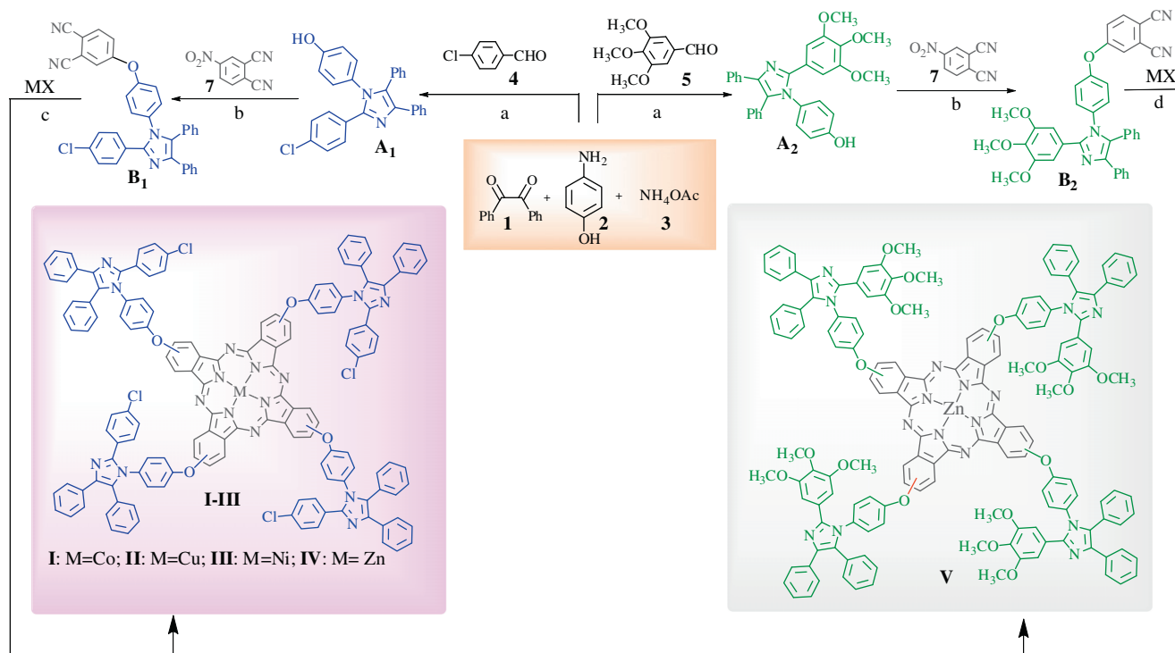
Scheme 1. Synthesis of metallophthalocyanines I–V . Reagents and conditions: (a) WD/SiO 2 , 140 °C (A 1 ): 72%, (A 2 ): 65%; (b) K 2 CO 3 , DMF, 24 h, rt, (B 1 ): 83%, (B 2 ): 89%; (c) metal salt (MX), DBU, DMAE, N 2 , reflux, (I): 34%, (II): 36%, (III): 35%, (IV): 41%; (d) Zn(OAc) 2 , DBU, DMF, N 2 , reflux (V): 33%.
