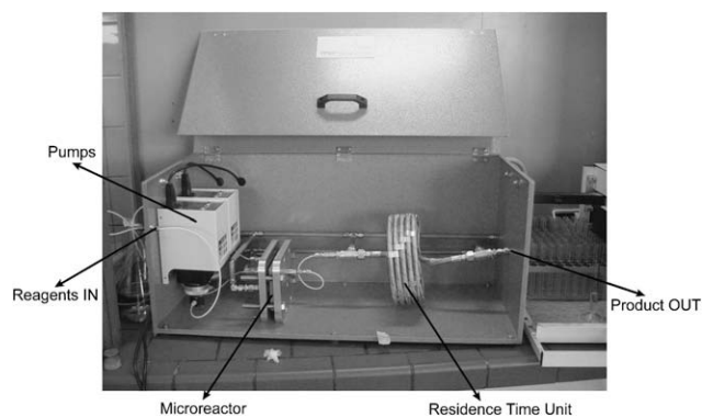
Figure 1. The applied microreactor: a CYTOS® College System, produced by CPC—Cellular Process Chemistry Systems GmbH; (1) input reagents via two pumps; (2) microreactor; (3) residence time unit; (4) output reaction mixture.
