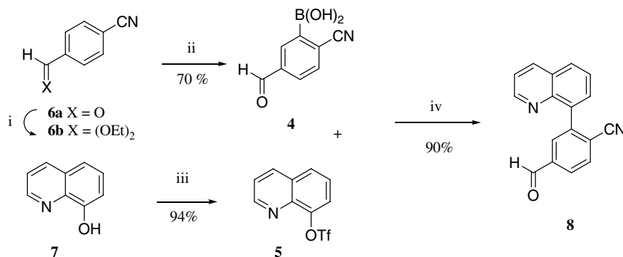
Scheme 1. Reagents and conditions: (i) triethyl orthoformate, ethanol, reflux; (ii) LiTMP, B(O- i Pr) 3 , THF, –60 °C; (iii) Tf 2 O, pyr, –5 °C and (iv) KF, toluene/methanol, cat. Pd(OAc) 2 , cat. biphenyl-2-dicyclohexyl-phosphane, 68 °C.
