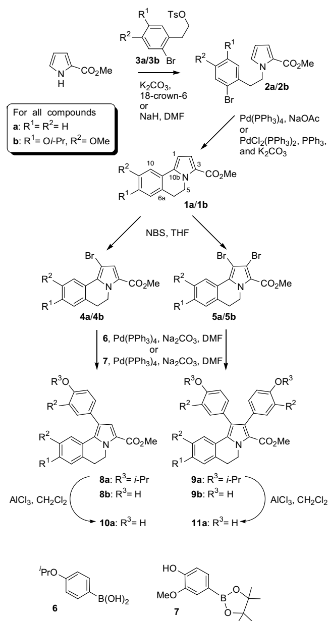
Scheme 1. Synthetic sequences.
