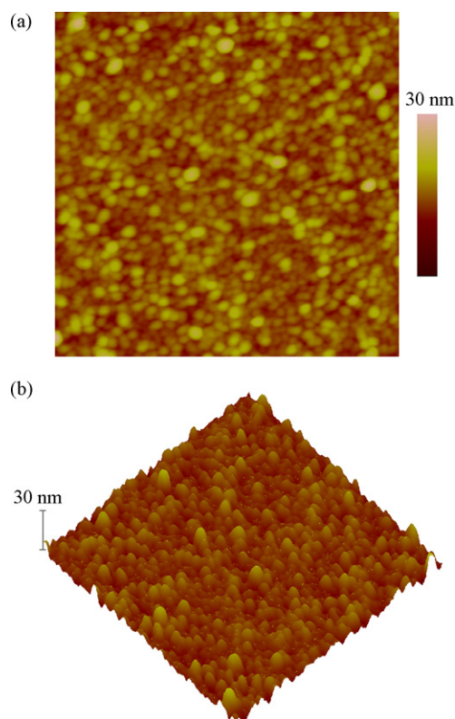
Fig. 2. (a) A topography of the Mg 0.1 Zn 0.9 O thin film. (b) A stereoscopic profile of the topography. The scan size is 1 \mu\text{m} \times 1 \mu\text{m} .
