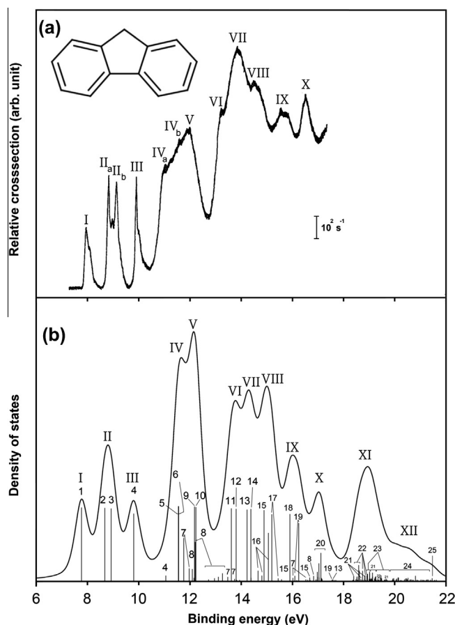
Fig. 1. Comparison of (a) the He (I) ultra-violet photoelectron spectrum with (b) the ADC(3)/cc-pVDZ ionization spectrum (FWHM = 0.6 eV) of fluorene. See Table 1 for detailed orbital assignment.
