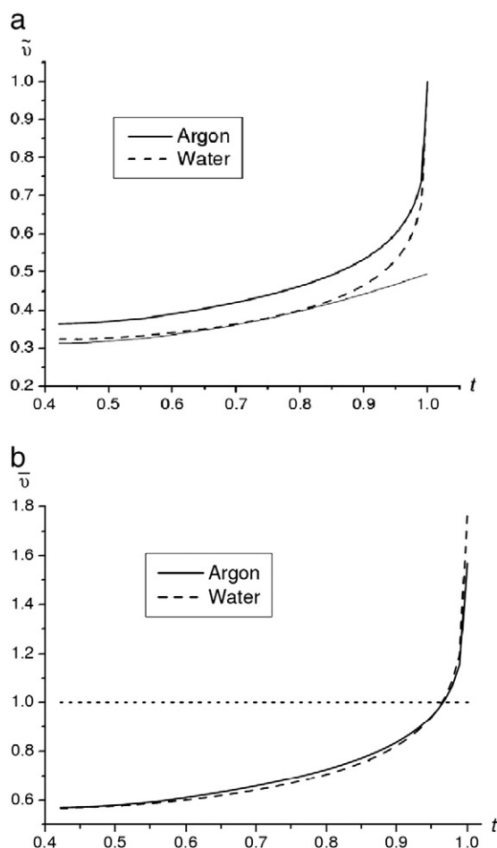
Fig. 2. Temperature dependencies of the normalized fraction volume for water and argon: a) \tilde{\nu}(t) = v(t)/v_c , b) \tilde{\nu}(t) = v(t)/v_R . The light line in a) corresponds to 0.86 \cdot \tilde{\nu}_R^{(Ar)}(t) (taken from [12]).
