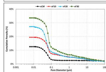
Reduced porosity due to NS incorporation
