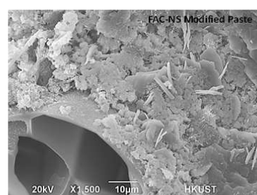
Denser Microstructure and Better Interface Properties
