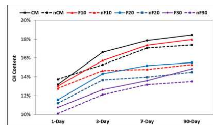
Enhanced pozzolanic activity with NS addition
