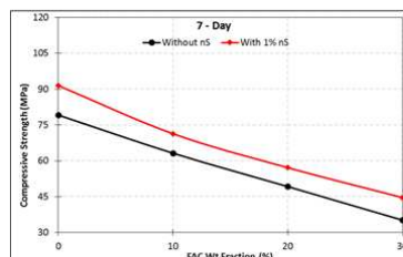
Compressive strength enhancement due to NS addition
