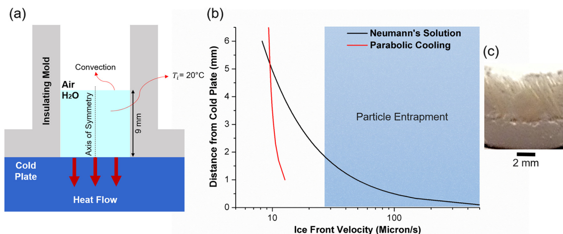
Fig. 1. (a) Schematic of directional freezing setup comprised of insulating side walls and conductive base (b) Predicted ice front velocities as a function of distance from the cold plate based on constant and changing boundary conditions (c) Sample chilled by constant cold plate temperature, showing a physical demarcation. (For interpretation of the references to color in this figure, the reader is referred to the web version of this article.)
