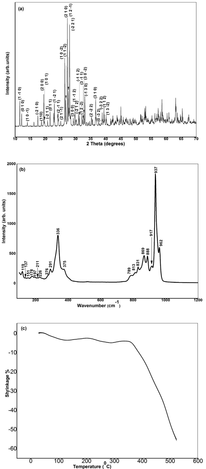
Fig. 1. (a) The X-ray diffraction pattern of Na _2 Zn _5 (MoO _4 ) _6 ceramics sintered at 590 °C for 1 h; (b) Raman spectrum of Na _2 Zn _5 (MoO _4 ) _6 ceramics sintered at 590 °C for 1 h; (c) Shrinkage behaviour of Na _2 Zn _5 (MoO _4 ) _6 ceramics.
