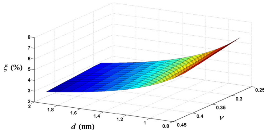
Fig. 1. Prediction of shear band dilatation \xi with the changes of diffusion distance d of free-volume and Poisson's ratio \nu .
