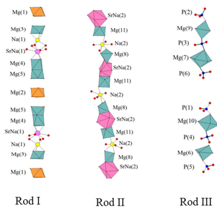
Rods I, II and III in \text{Na}_3\text{SrMg}_{11}(\text{PO}_4)_9
