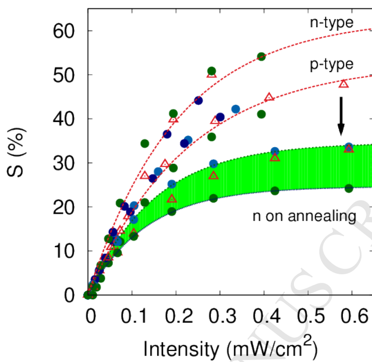
Plot shows the variation in film sensitivity with incident light intensity.
