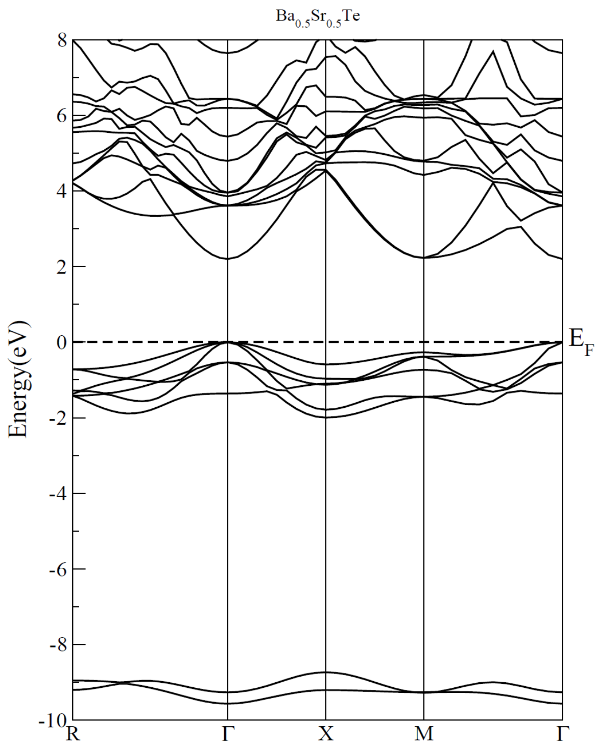
Electronic band structure of the \text{Ba}_{0.50}\text{Sr}_{0.50}\text{Te} ternary alloy
