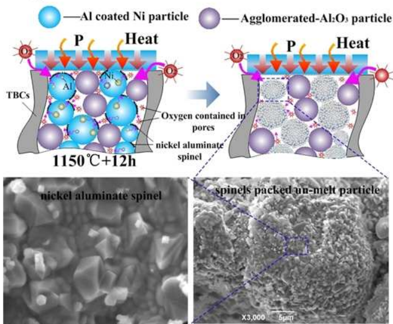
(b) Schematic formation of A- \text{Al}_2\text{O}_3 /Ni-Al sealed films
