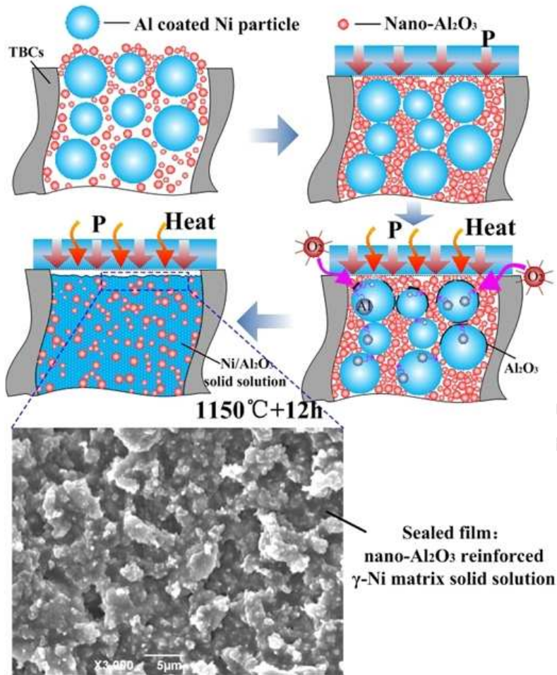
(b) Schematic formation of A- \text{Al}_2\text{O}_3 /Ni-Al sealed films
