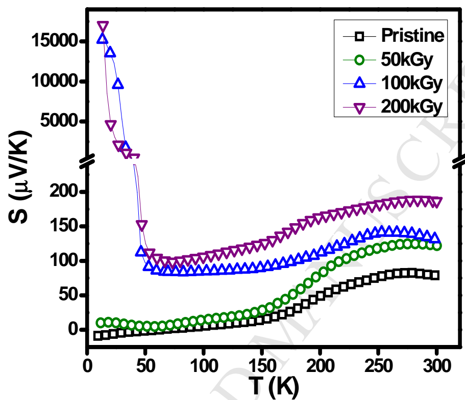
Figure: Temperature dependent S(T) for various electron beam dosages
