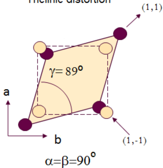
Triclinic distortion
