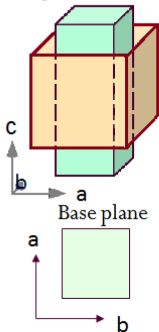
Tetragonal distortion
