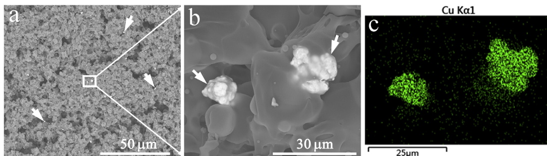
Fig. 2. FESEM pictures and EDX analyses of the as-sprayed polyimide-Cu coatings showing even distribution of copper particles in polyimide matrix and enwrapping state of the particles by polyimide. The white arrows point to typical copper particles seen on the top surfaces of the coatings.
