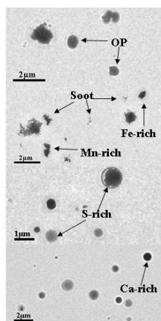
TEM images of particles from gasoline engines
