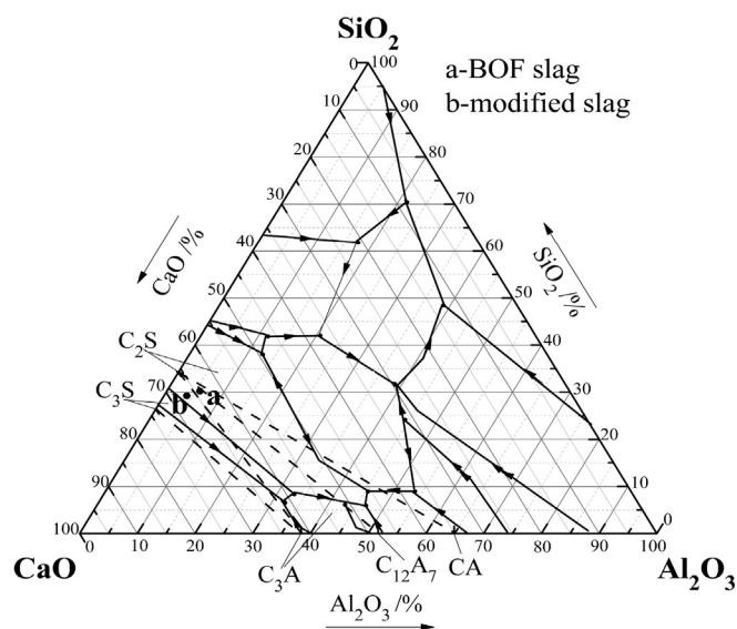
Fig. 1. The chemical composition of BOF slag and modified slag located in CaO-SiO 2 -Al 2 O 3 ternary phase diagram.
