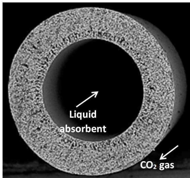
Affordable kaolin-alumina hollow fiber membrane contactor
