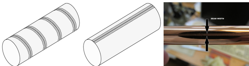
Fig. 2. Different adhesion styles of straw construction; (Left) the original doubly-wound style, (Centre) the new straight-adhesion style, (Right) the welding seam of a completed straw.
