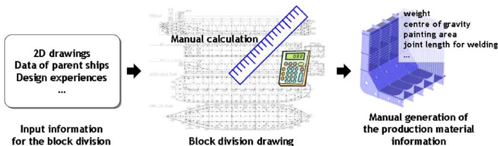
Fig. 2. Existing procedure of manually generating the production material information at the initial process planning stage.
