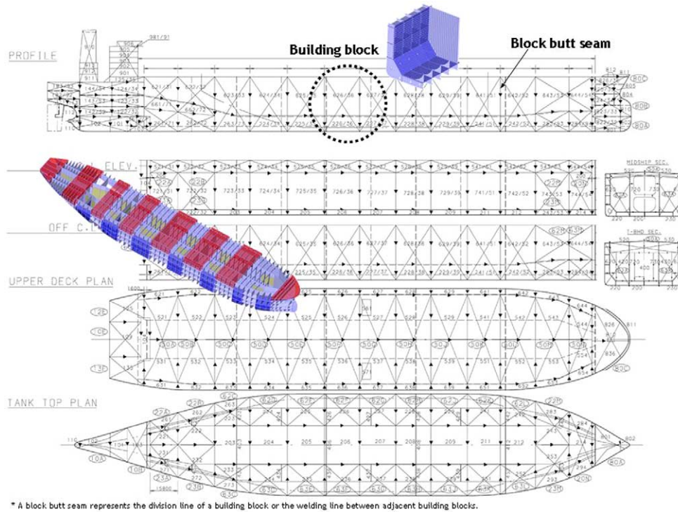
Fig. 1. Example of the block division drawing of the 300 K VLCC.
