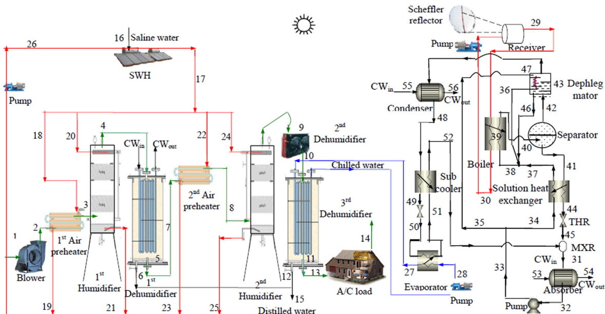
Fig. 1. Two stage desalination and cooling plant.
