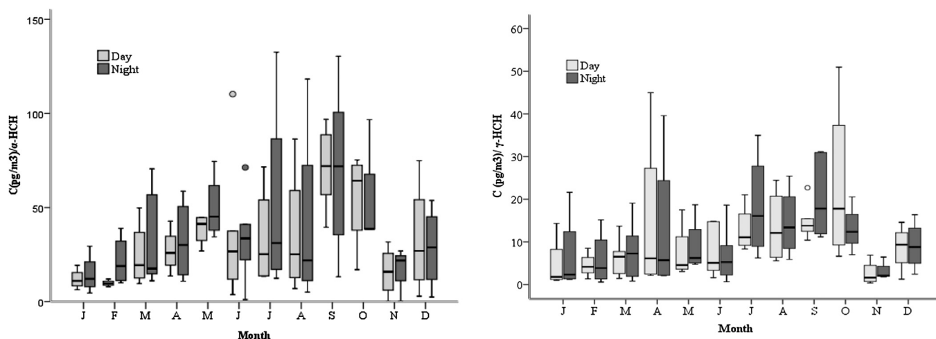
Fig. 1. Monthly variations in \alpha -HCH (left panel) and \gamma -HCH (right panel) concentrations in gas phase.
