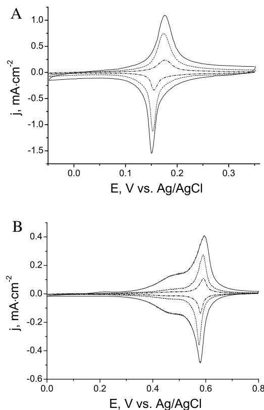
Fig. 1. Cyclic voltammograms of (a) Prussian Blue: 0.90 nmol cm -2 (dash-dot line), 2.45 nmol cm -2 (short dash line), 4.05 nmol cm -2 (solid line) and (b) nickel hexacyanoferrate: 0.40 nmol cm -2 (dash-dot line), 1.15 nmol cm -2 (short dash line), 4.10 nmol cm -2 (solid line); in 0.1 M KCl and 0.1 M HCl, sweep rate 40 mV s -1 .
