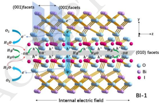
Fig. Photocatalytic mechanism diagrams of highly active (010) facets for BI-1
